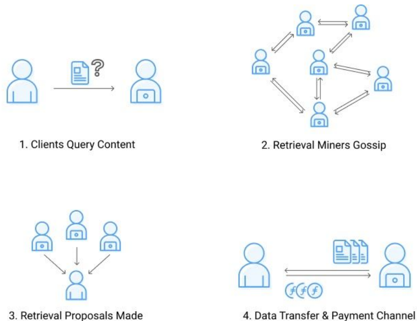
Figure 11: Content delivery flow on Filecoin
